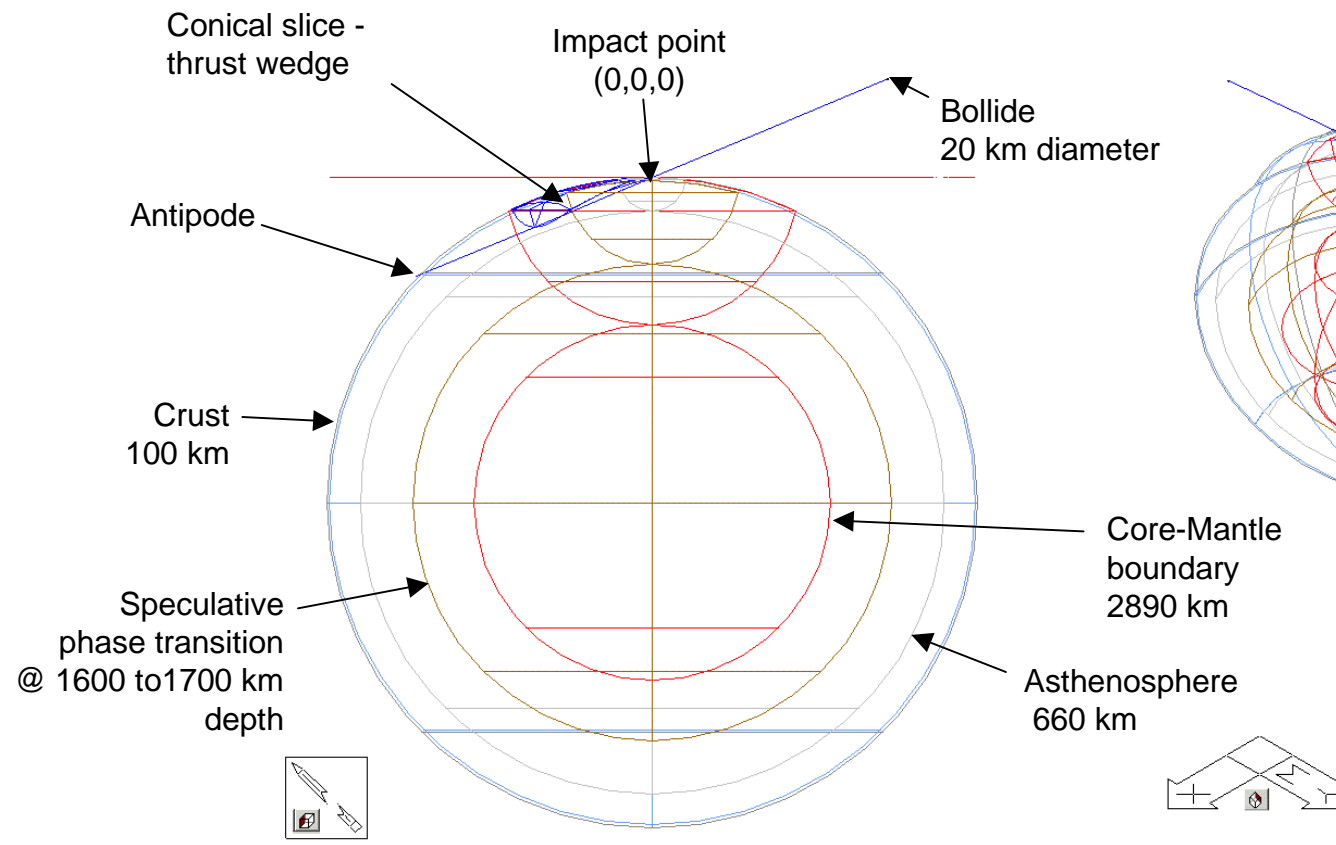
PROFILE VIEW
