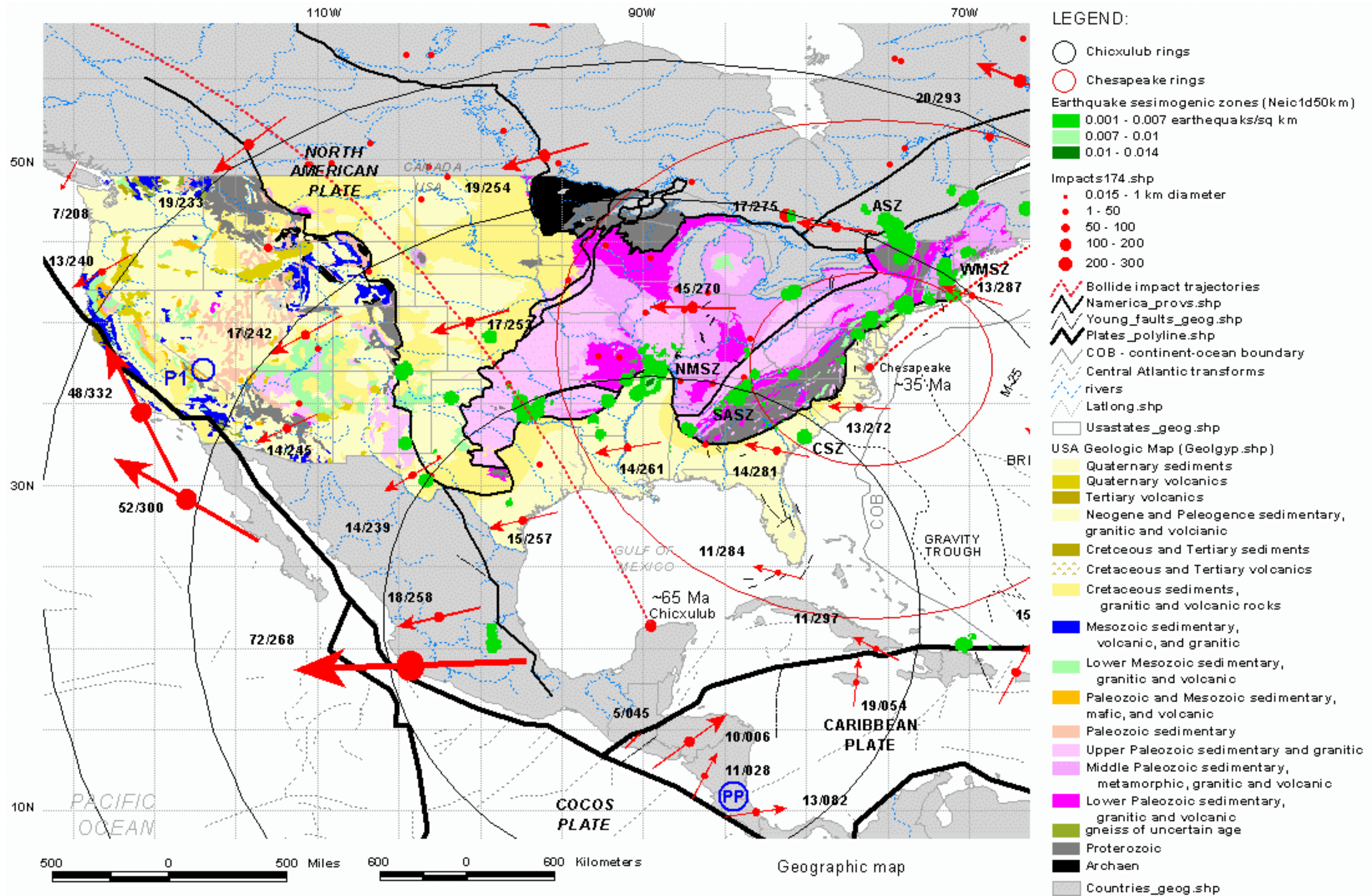
Plate boundaries, NASA GPS horizontal plate-motion vectors, seismicogenic zones, and proposed multi-ring structures stemming from the Chicxulub and Chesapeake impacts with respect to physiographic regions of North America and a generalized geological map of the United States
